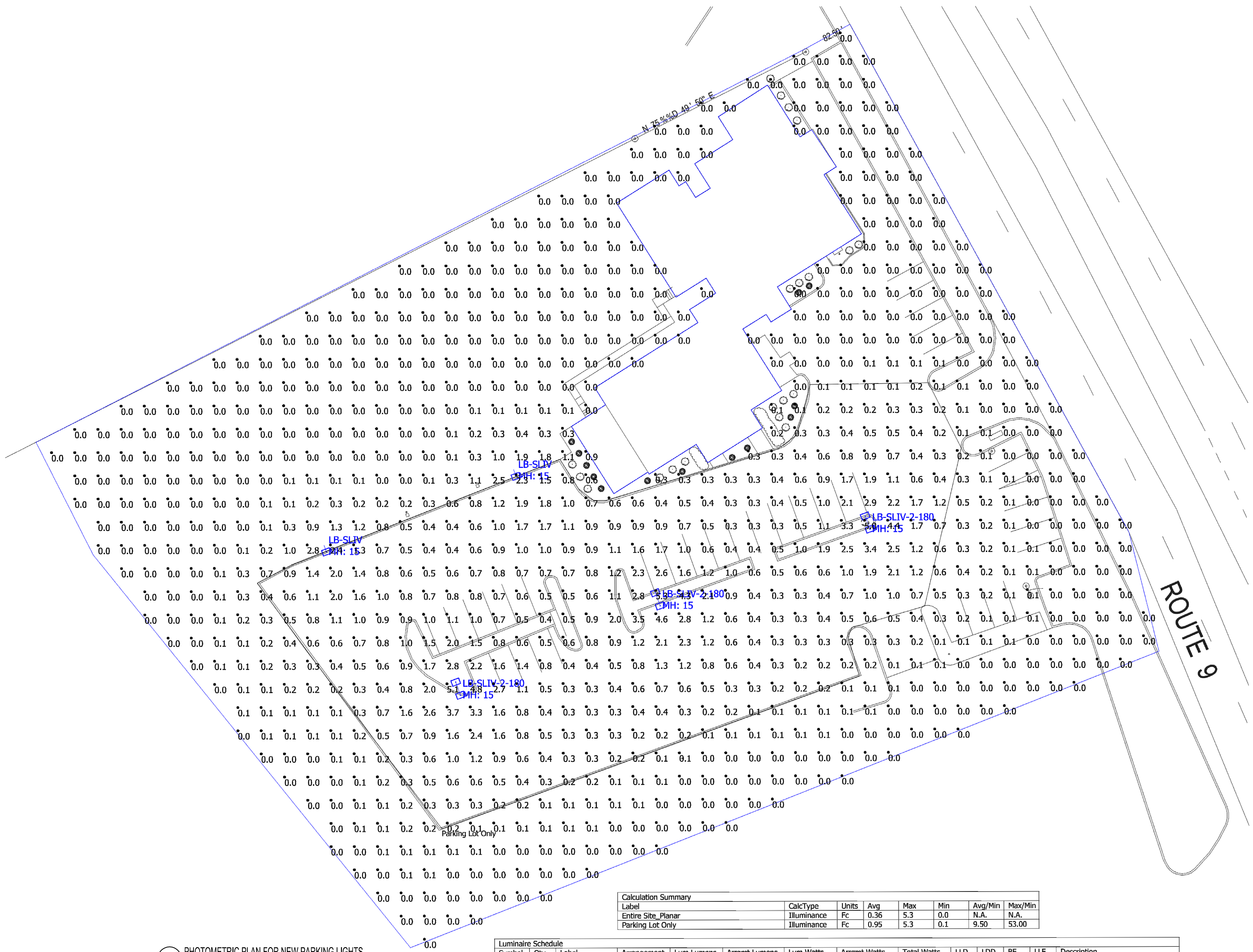
1 PHOTOMETRIC PLAN FOR NEW PARKING LIGHTS SCALE: 1"=20'-0"
